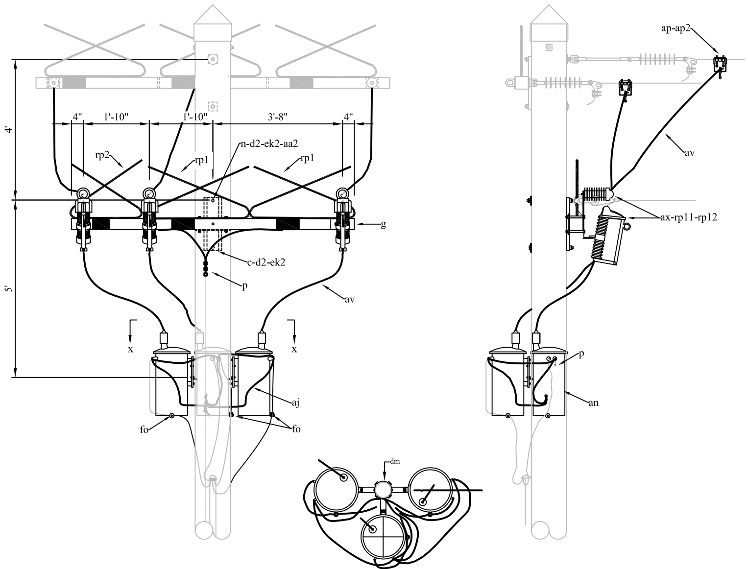
SECTION X-X
